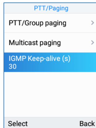
Figure 75: IGMP setting
