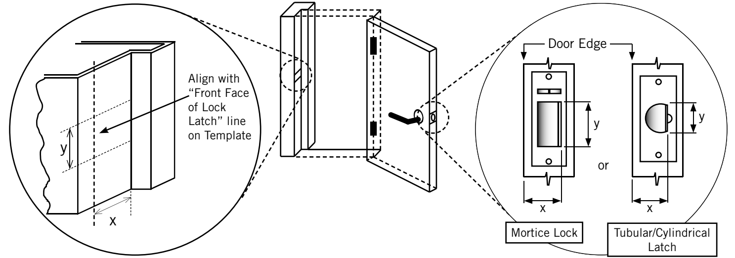
Fig. 2 - 100C/110C Series Euro Face Plate Type "C" Template Outline
