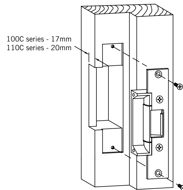
Fig. 4 - Wood Jamb Installation
