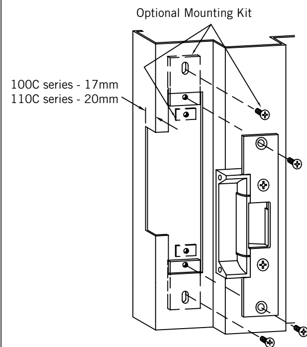
Fig. 3 - Metal Jamb Installation
