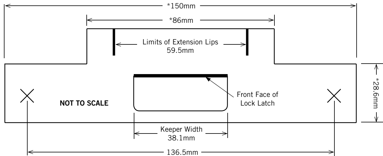
Fig. 2 - 100C/110C Series Euro Face Plate Type "C" Template Outline
