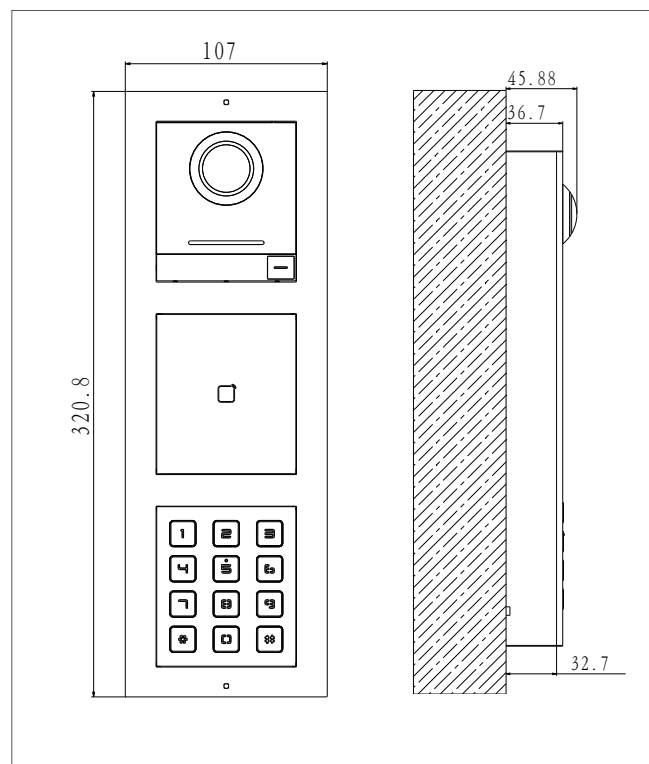
Three Modules Surface Mounting
