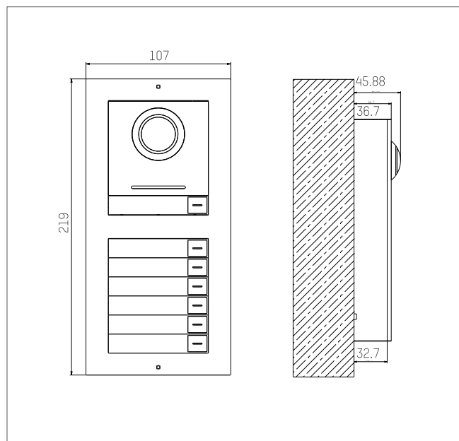
Dual Modules Surface Mounting
