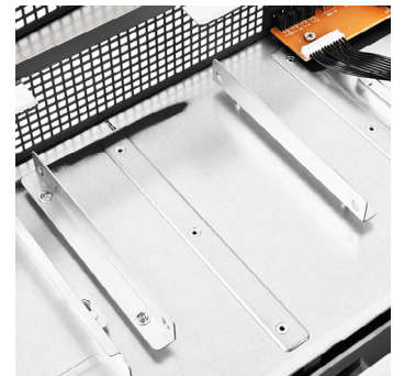
3.5" devices cage
