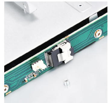
6 Gb/s Mini-SAS SFF-8087
