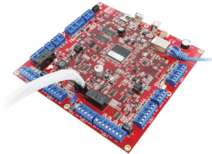
996035PCB&K Integriti IAC Controller PCB
