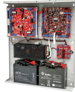
IAC Controller shown in 8 Door configuration.
